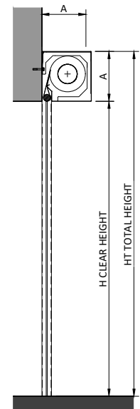
TYPICAL SECTION FACE FIXED
